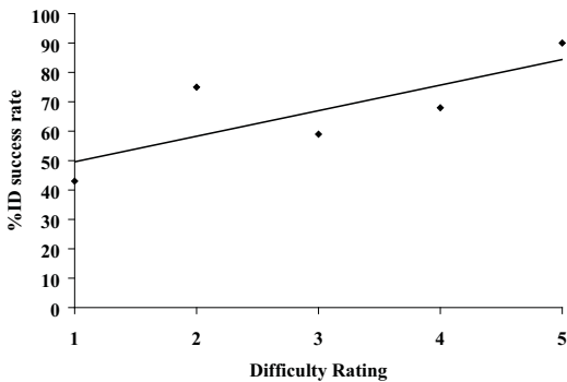
Figure 3. Effect of the degree of difficulty in correctly identifying pairs of photographs.
