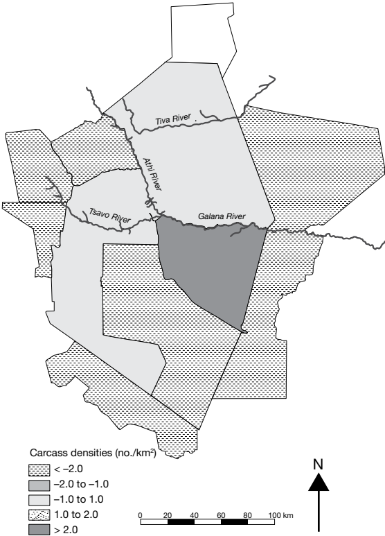
Figure 8. Elephant carcass densities (no./km 2 ) in the Tsavo–Mkomazi ecosystem (early February 2011).
